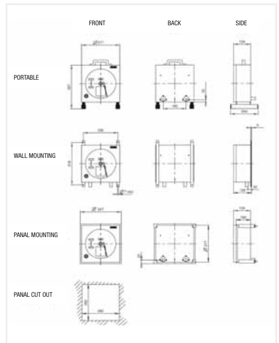
Dimensional Data MX 4888SST (mm)
